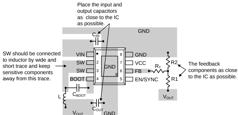
Figure 8 (b). PCB Layout Guide for SOP-8 (Exposed Pad)
