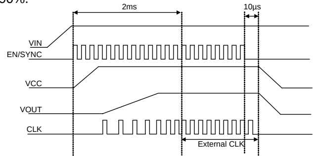
Figure 6. Startup Sequence Using External Sync Clock
