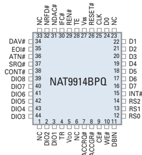
Figure 2. NAT9914BPQ
