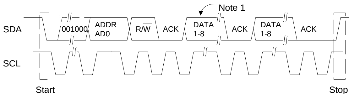
Figure 6. Control Port Timing, I²C Mode
