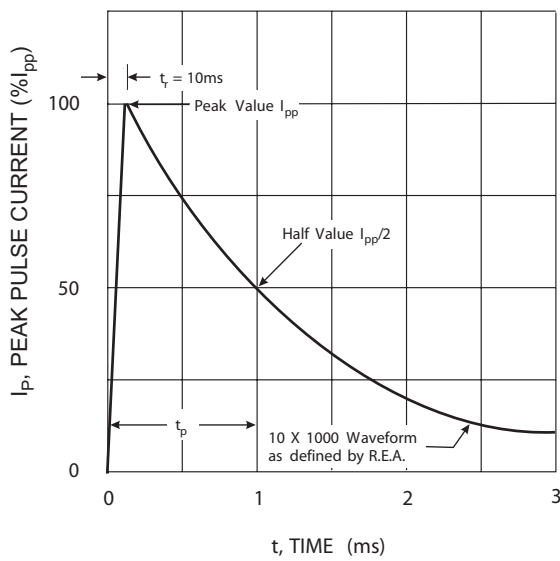
Fig. 1 Pulse Waveform
