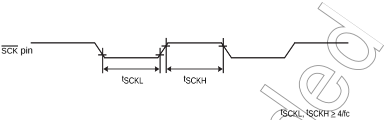
Figure 10-3 External Clock
