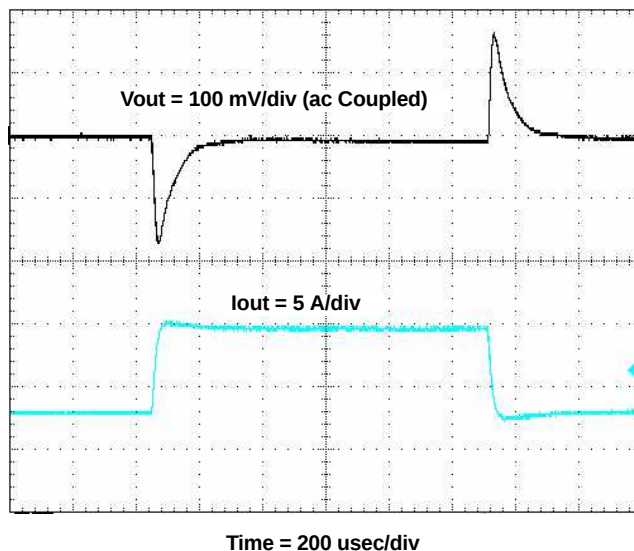
Figure 4. Load Transient Response, TPS54073
