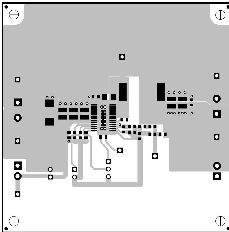
Figure 11. Top-side Layout
