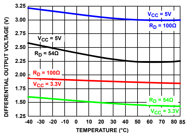
FIGURE 13. DRIVER DIFFERENTIAL OUTPUT VOLTAGE vs TEMPERATURE
