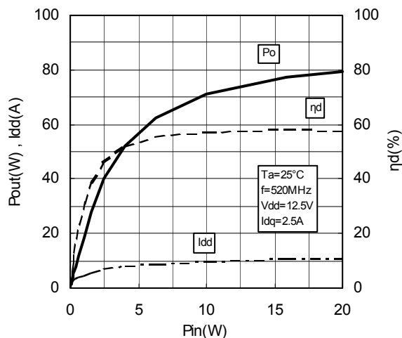
Pin-Po CHARACTERISTICS
