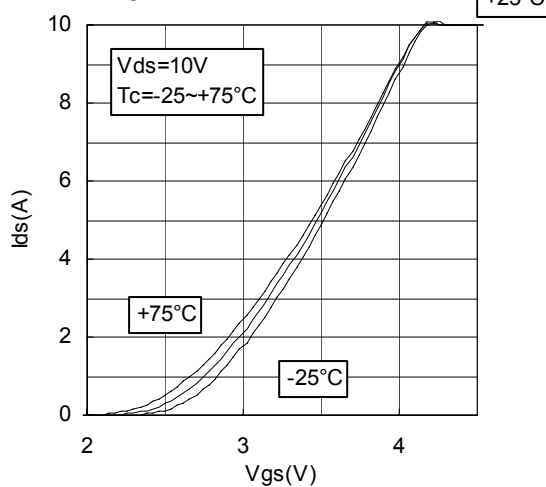
Vgs-Ids CHARACTERISTICS 2
