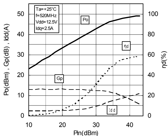
Pin-Po CHARACTERISTICS
