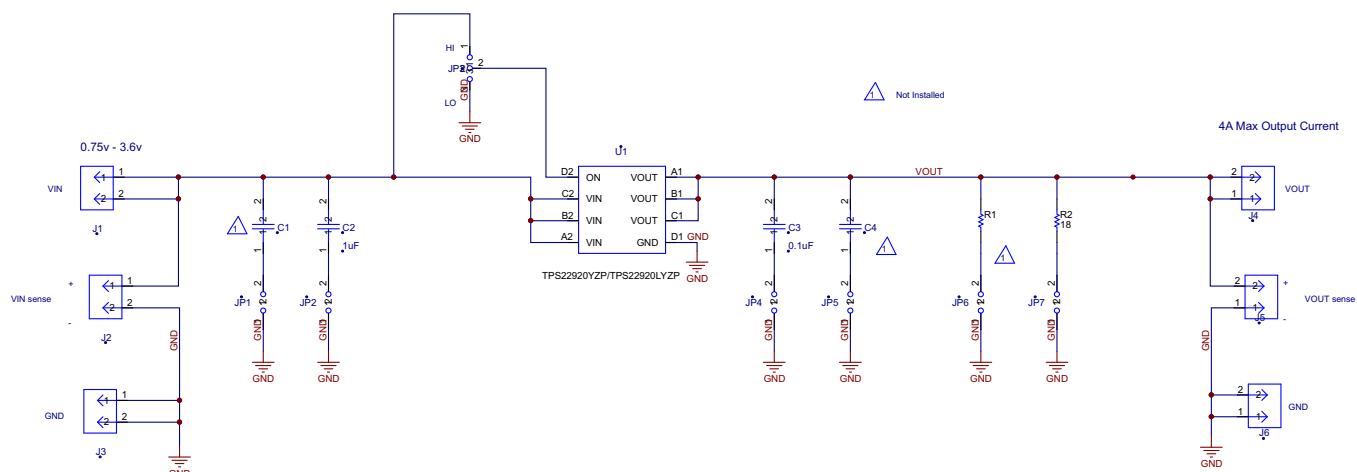
Figure 4. TPS22920EVM-002 Schematic
