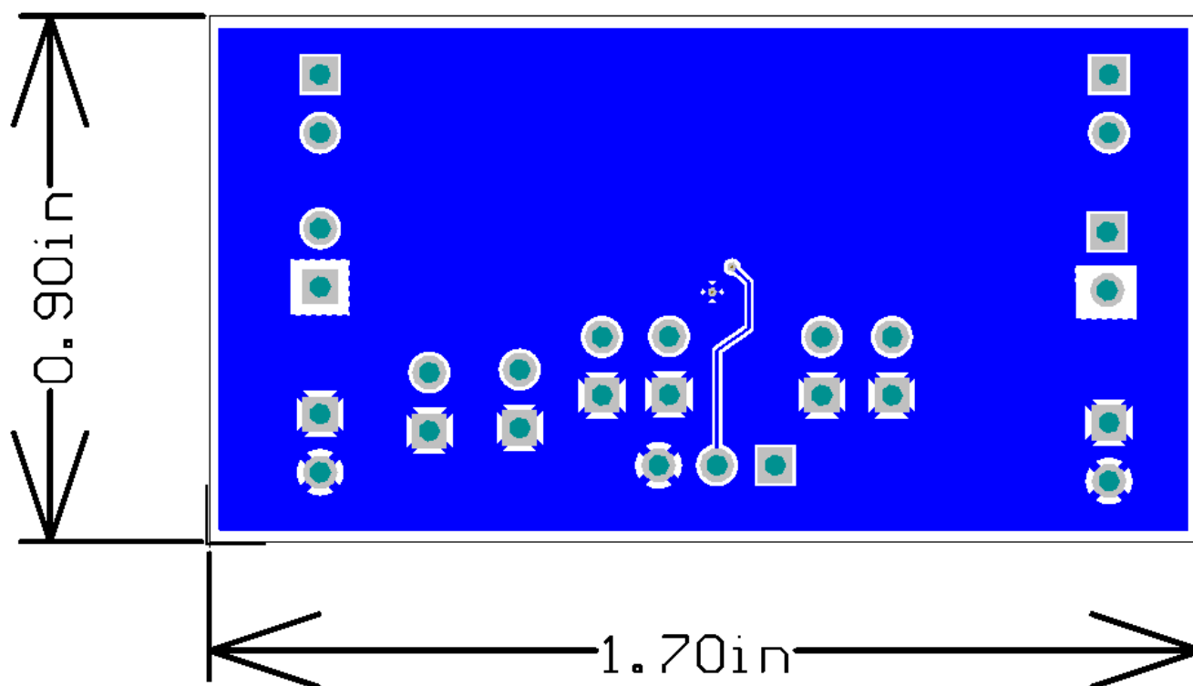
Figure 3. Bottom Layer
