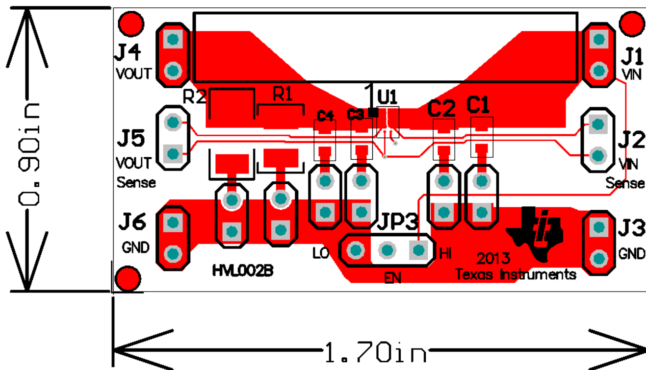
Figure 2. Top Layer
