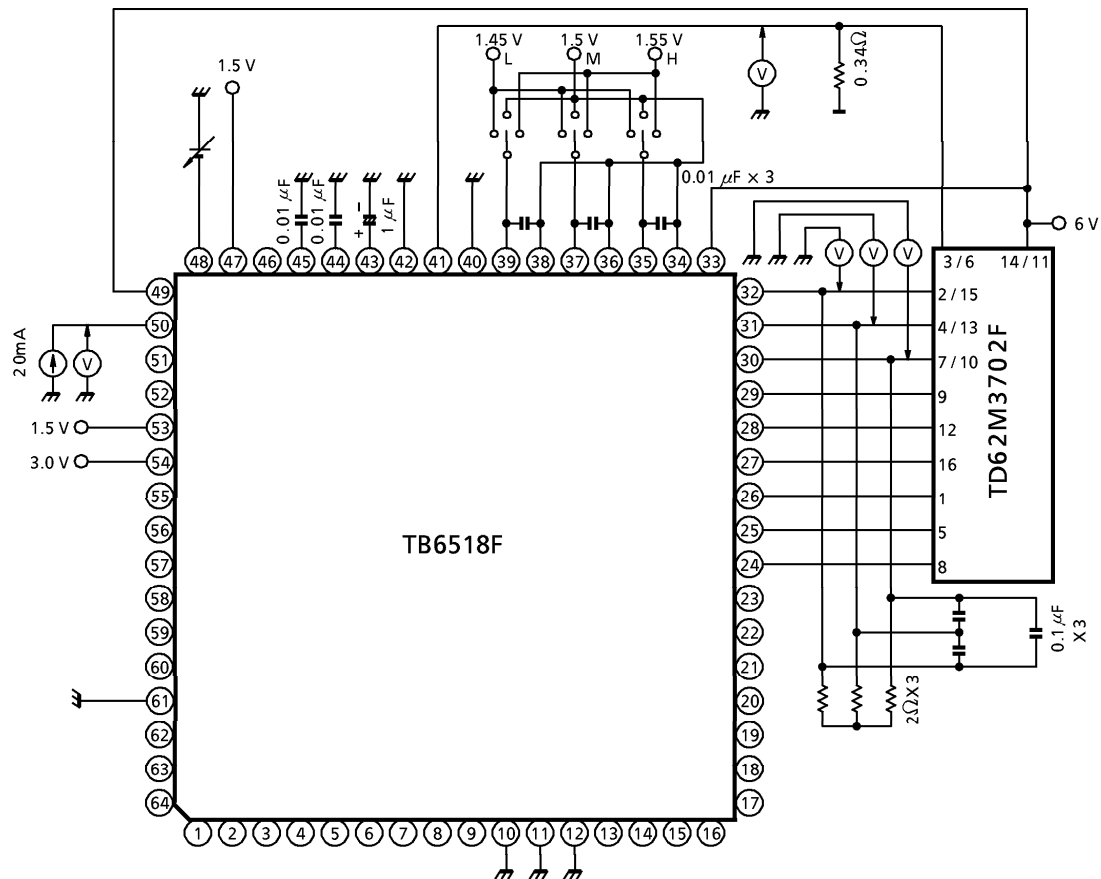
TEST CIRCUIT 11. CVLL (1), CVLL (2)
