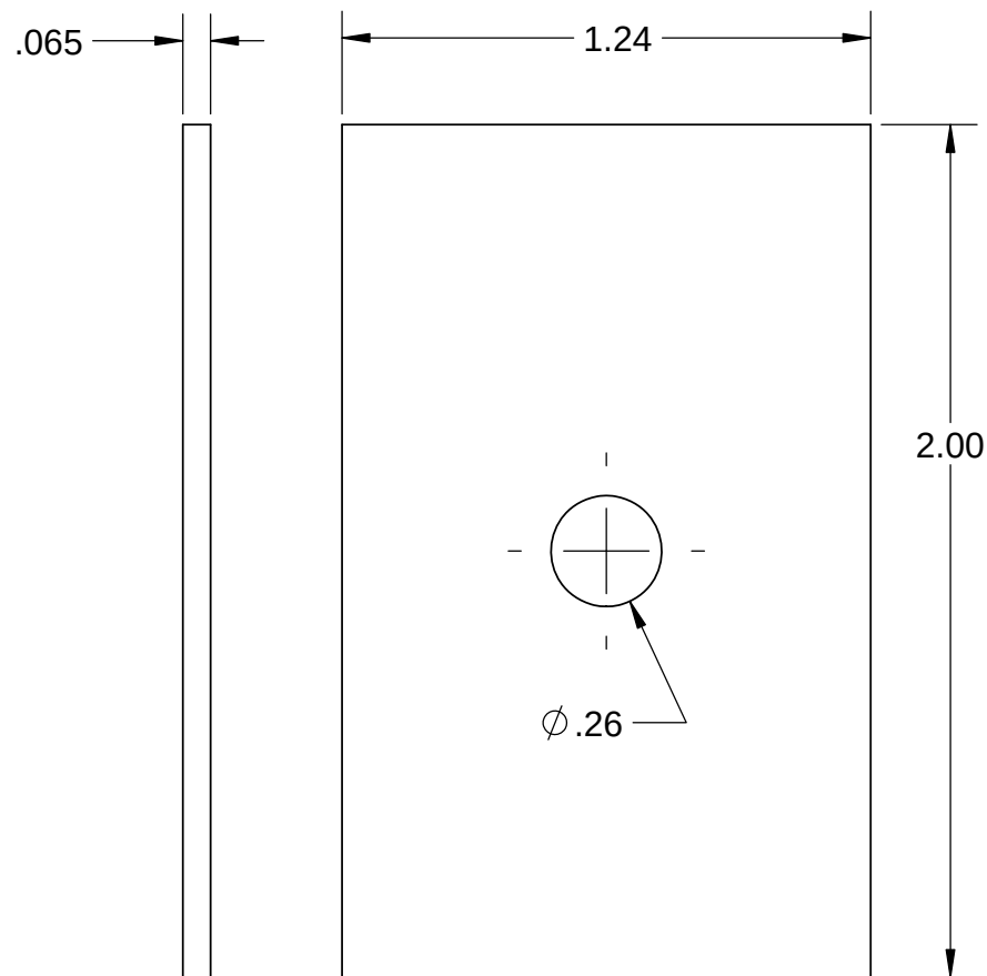
.065 board
