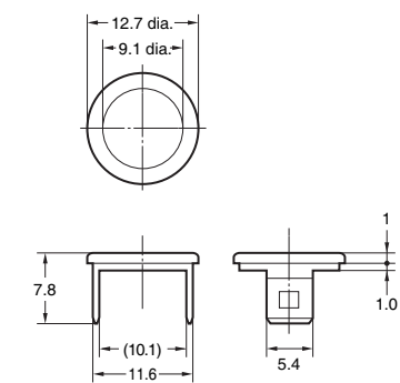
Flange (Round) A3A-25
