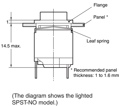
Panel Mounting Dimensions
