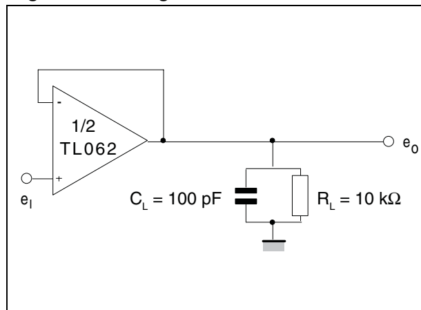
Figure 17. Voltage follower
