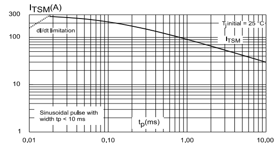
Figure 10: Non-repetitive surge peak on-state current
