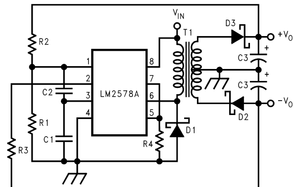
FIGURE 22. Buck-Boost Regulator
