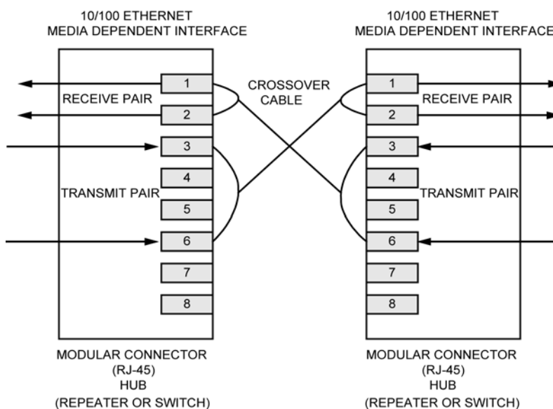
Figure 7. Typical Crossover Cable Connection
