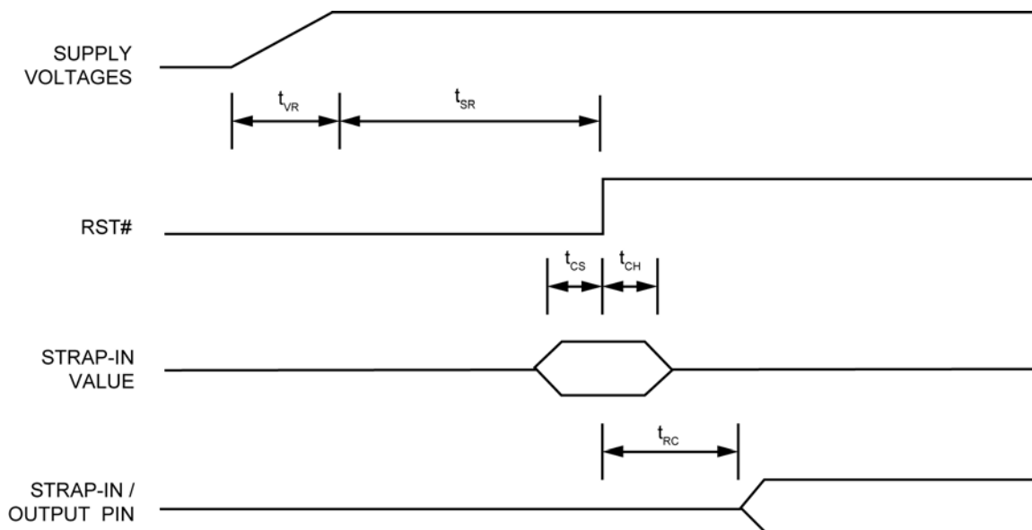
Figure 20. Power-Up/Reset Timing
