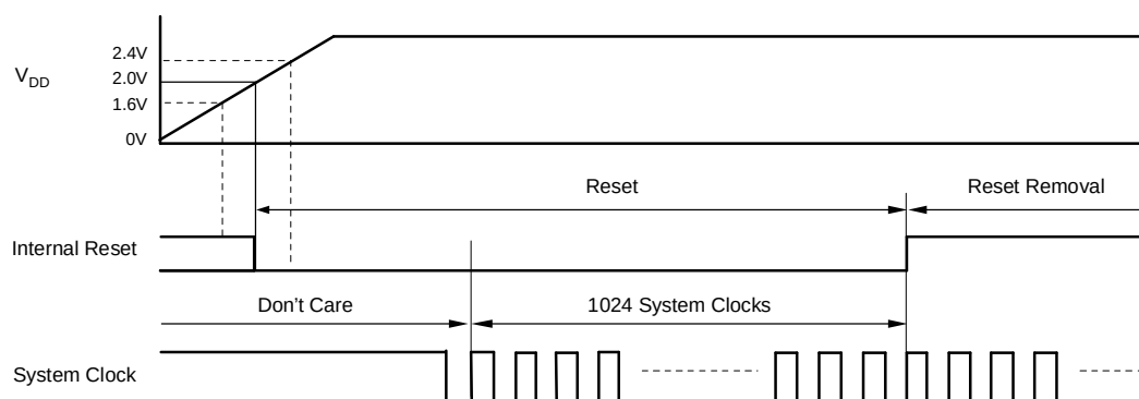
Figure 20. Power-On-Reset Timing
