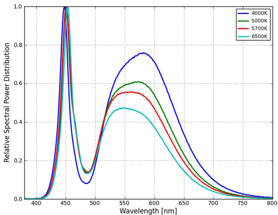
Figure 3a. Typical color spectrum of MXA7-PWxx emitter, integrated measurement at solder pad temperature = 25°C, forward current = 100 mA.
