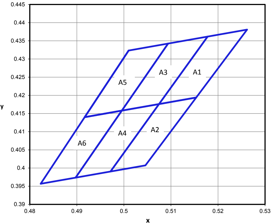
Figure 12. 2200K 1/6th color bin structure.
