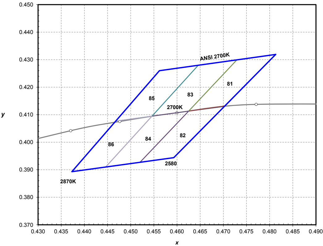
Figure 14. ANSI 2700K 1/6th color bin structure.
