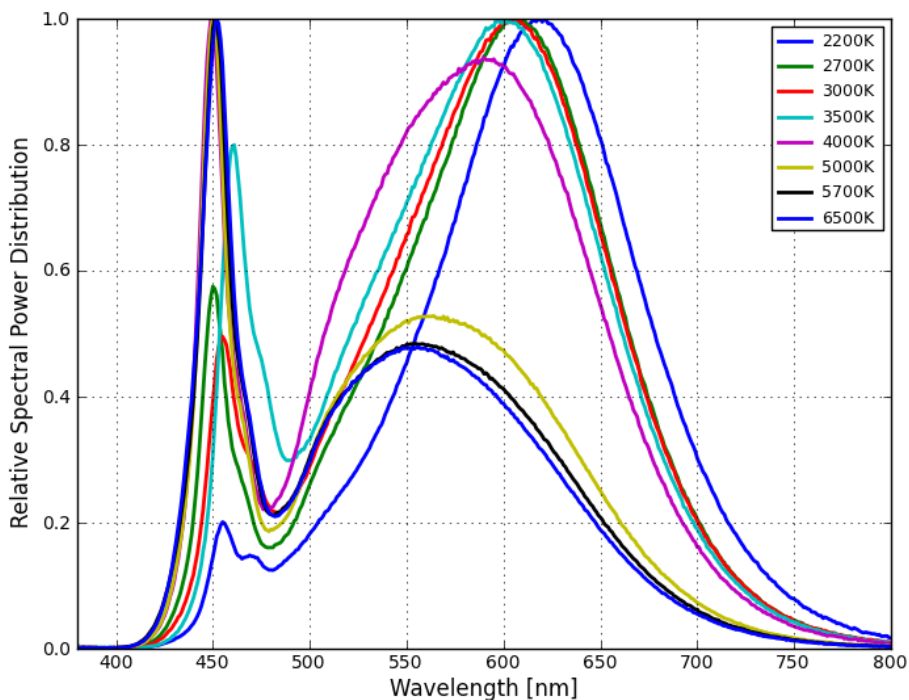
Figure 3b. Typical color spectrum of MXA8-PWxx emitter, integrated measurement at solder pad temperature = 25°C, forward current = 100 mA.
