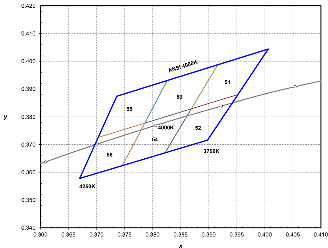
Figure 17. ANSI 4000K 1/6th color bin structure.
