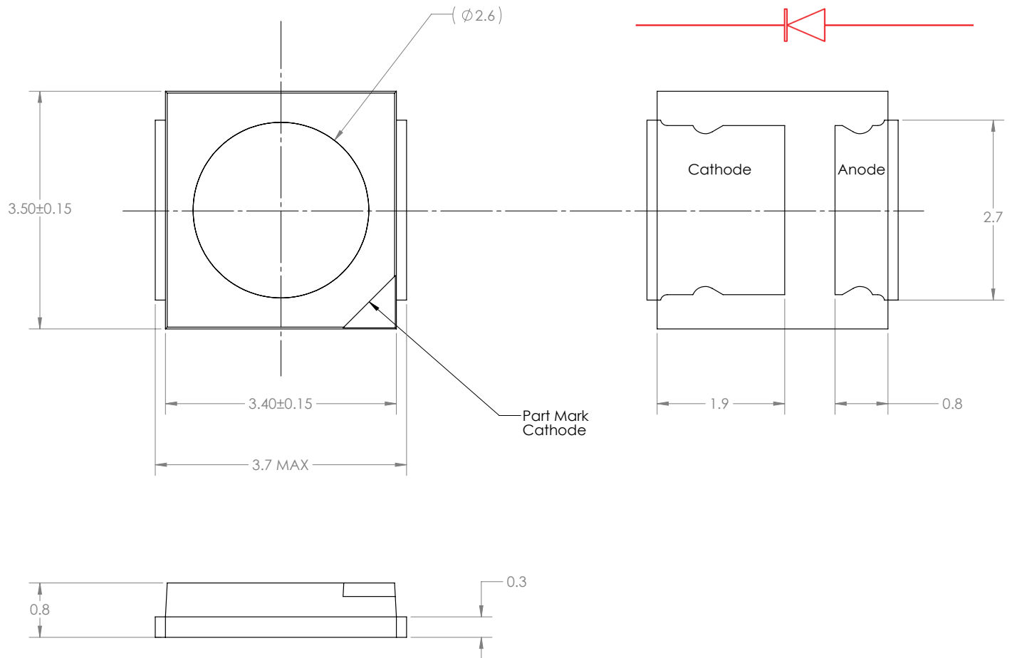
Figure 1. Package outline drawing.
