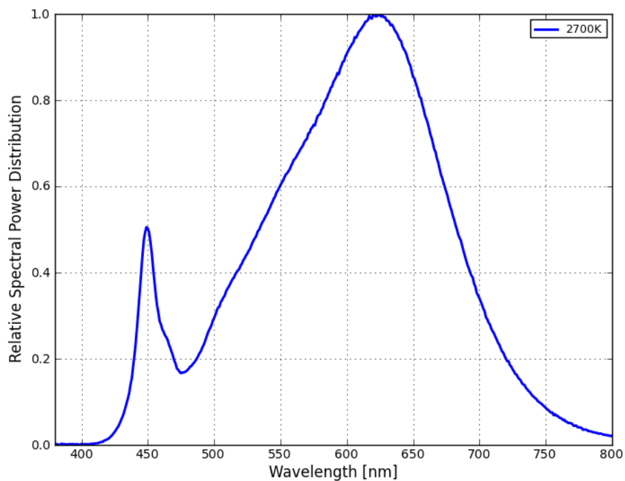
Figure 3c. Typical color spectrum of MXA9-PWxx emitter, integrated measurement at solder pad temperature = 25°C, forward current = 100 mA.
