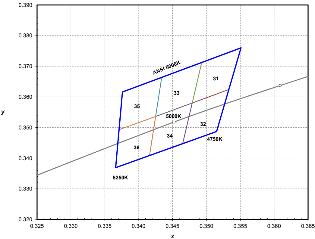
Figure 18. ANSI 5000K I/6th color bin structure.
