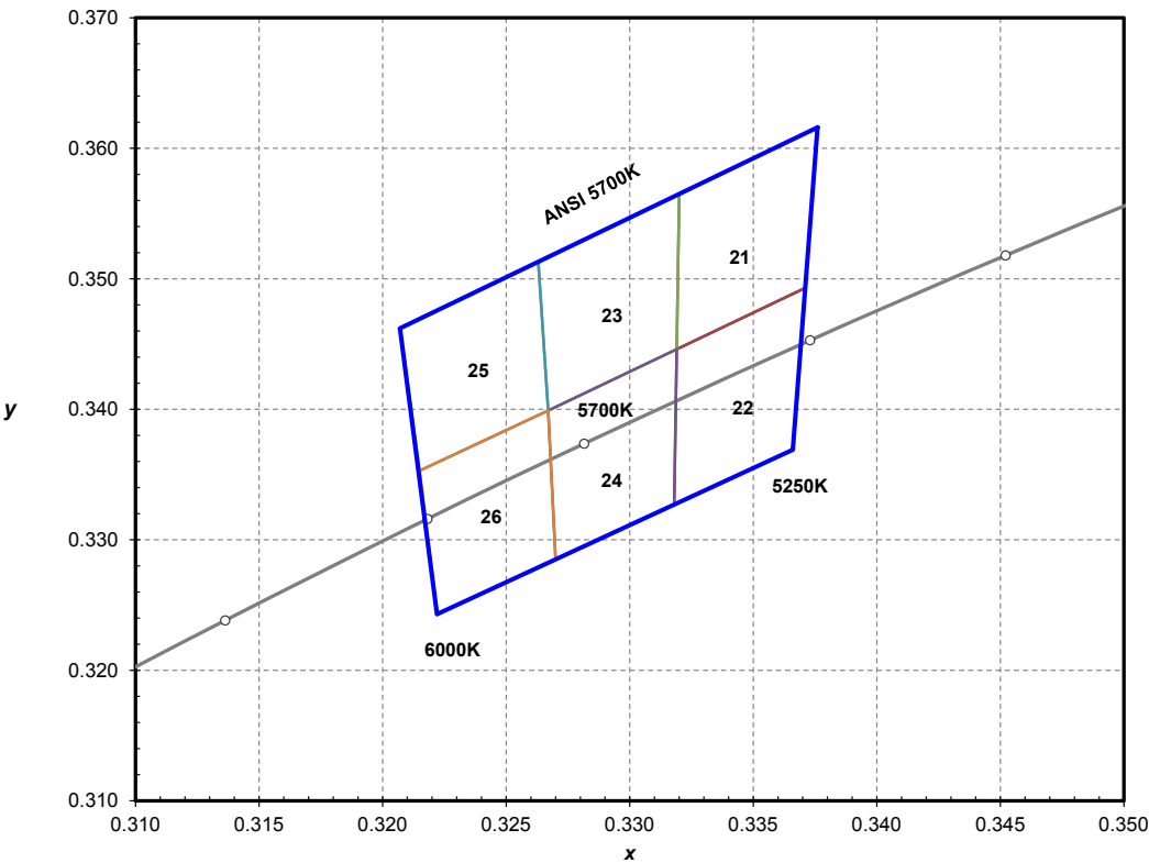
Figure 19. ANSI 5700K 1/6th color bin structure.
