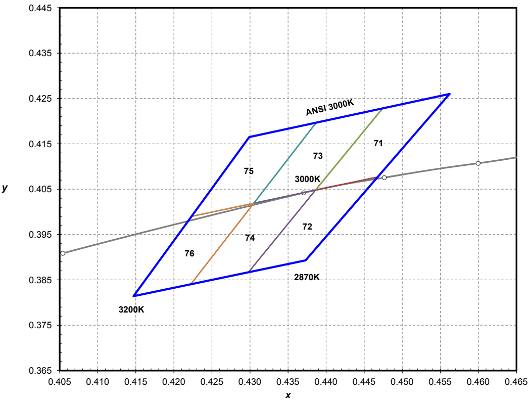
Figure 15. ANSI 3000K 1/6th color bin structure.
