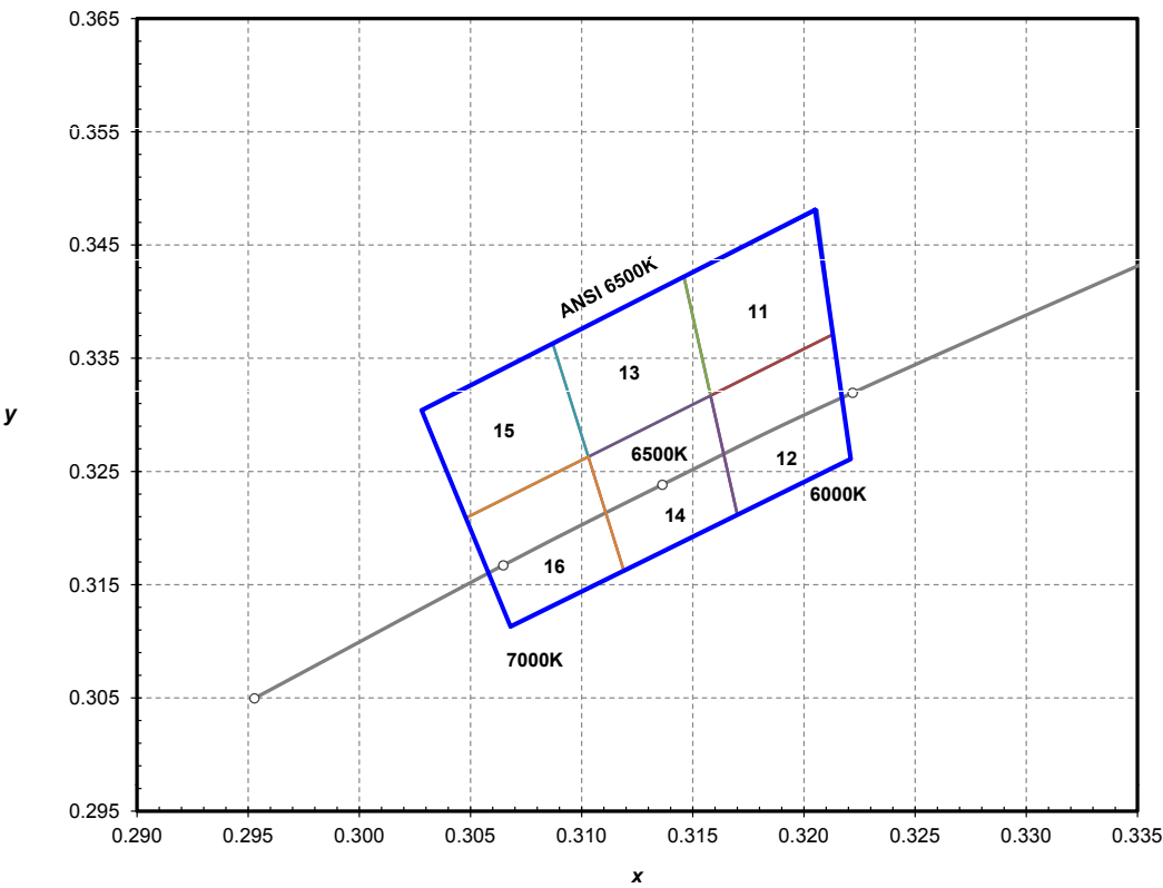
Figure 20. ANSI 6500K 1/6th color bin structure.
