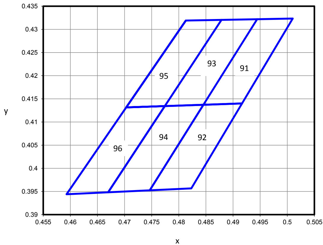
Figure 13. 2500K I/6th color bin structure.
