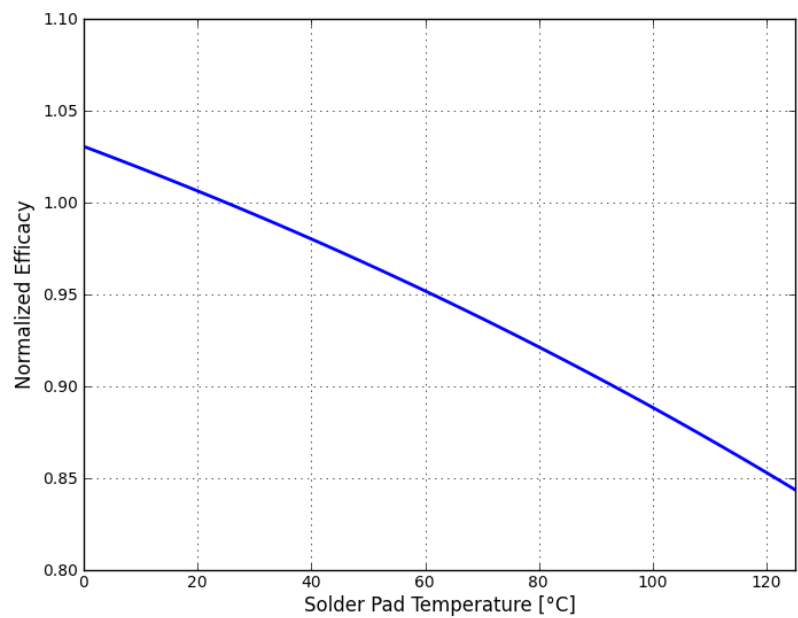
Figure 6. Typical relative emitter efficacy as a function of solder pad temperature.
