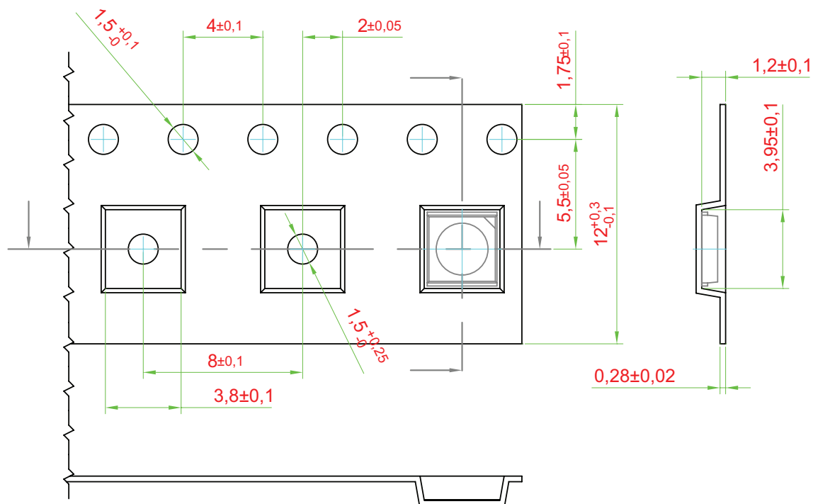
Figure 10. Emitter pocket tape packaging.
