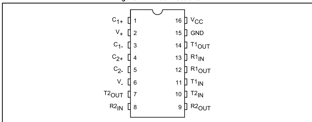
Figure 1: Pin connections
