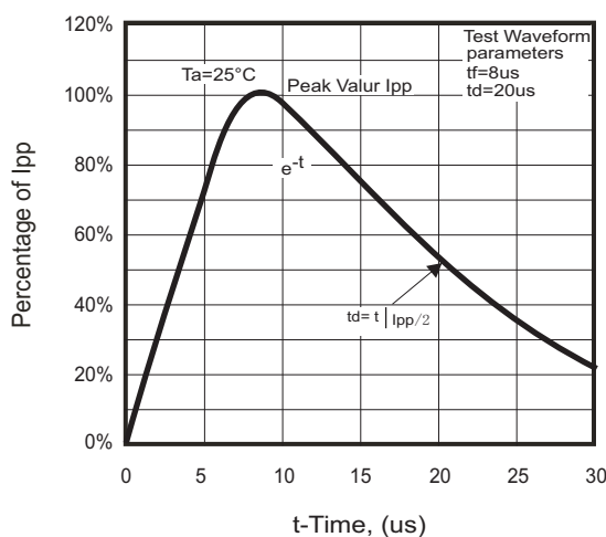
Fig.1 - Pulse Waveform
