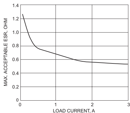
Figure 16. Stability
