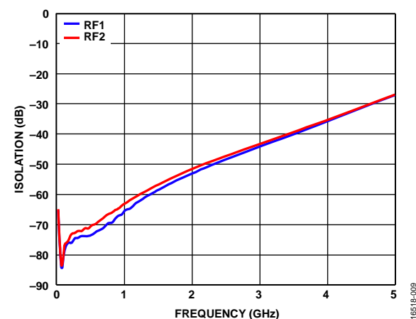
Figure 9. Isolation Between RF1 and RF2 vs. Frequency at V_{DD} = 5\text{ V}
