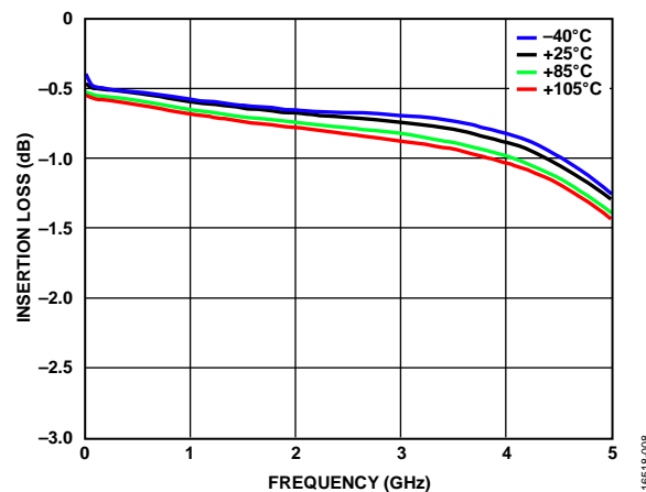
Figure 8. Insertion Loss vs. Frequency for Various Temperatures at V_{DD} = 5\text{ V}
