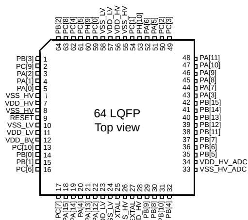
Figure 2. MPC560xB LQFP 64-pin configuration
