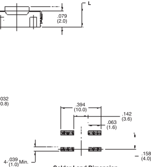
Solder Land Dimension
