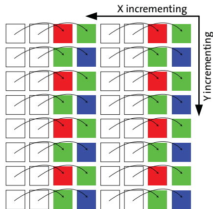
Figure 19: Pixel Readout (Column Bin 2X)
