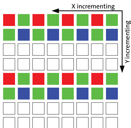
Figure 17: Pixel Readout (Row Skip 2X)
