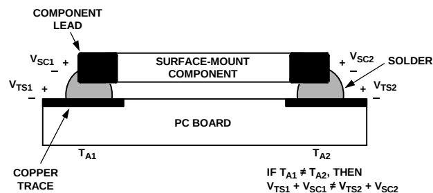
Figure 73. Mismatch in Seebeck Voltages Causes Seebeck Voltage Error
