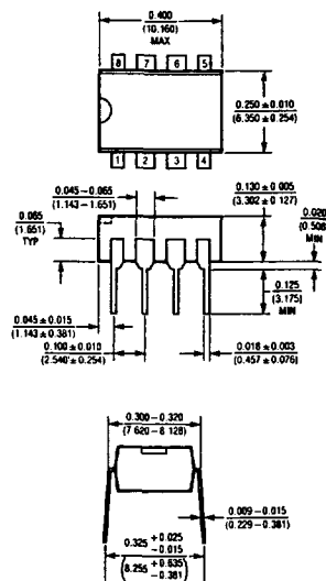
N Package 8-Lead Plastic DIP
