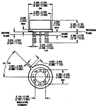
H Package 8-Lead TO-5 Metal Can
