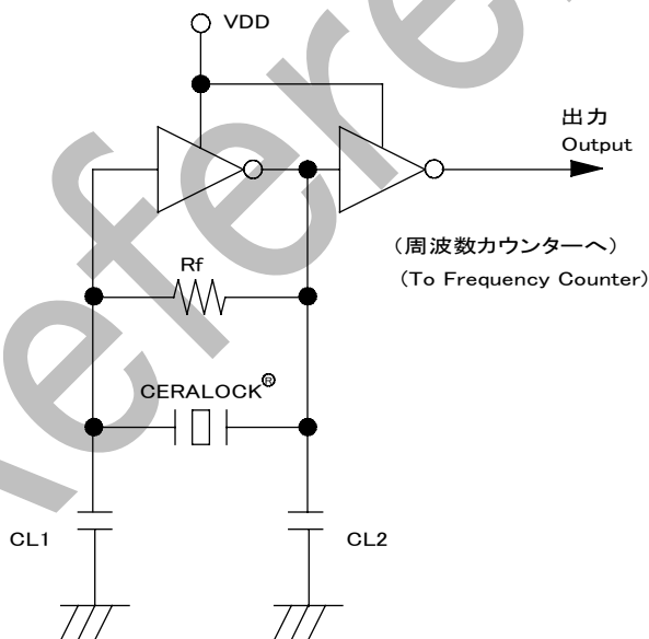
Figure 2. Test Circuit
