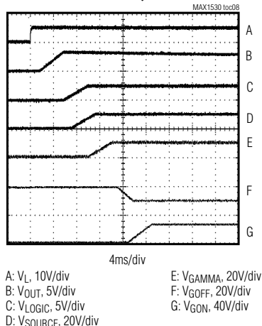
STARTUP SEQUENCE
