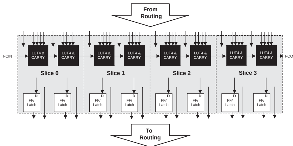
Figure 2-1. PFU Block Diagram
