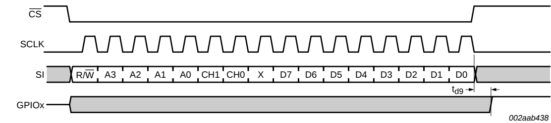
Fig 31. SPI write IOState to GPIO switch
