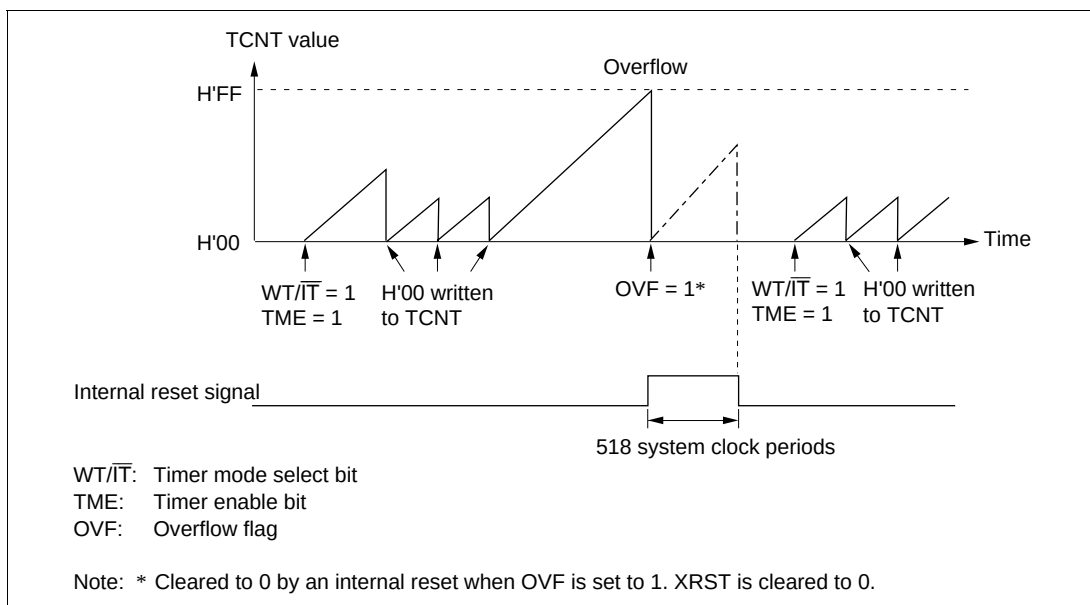
Figure 14.3 Operation in Watchdog Timer Mode
