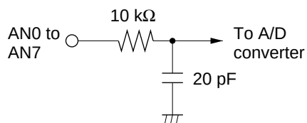
Figure 19.8 Analog Input Pin Equivalent Circuit
