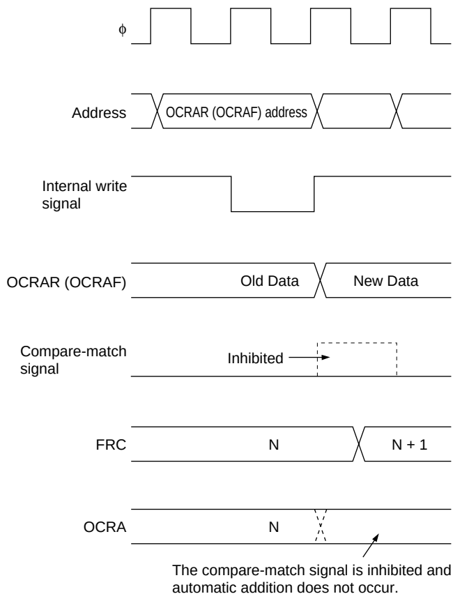
Figure 11.21 Contention between OCRAR/OCRAF Write and Compare-Match (When Automatic Addition Function Is Used)
