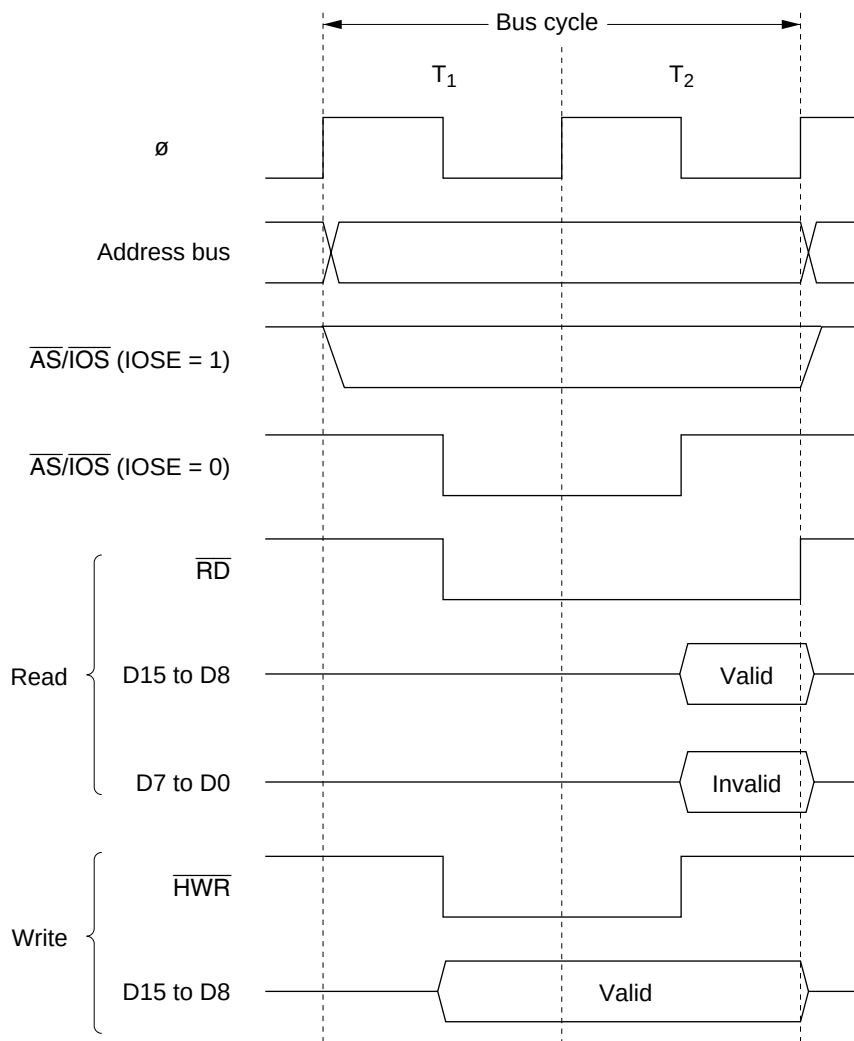
Figure 6.5 Bus Timing for 8-Bit 2-State Access Space
