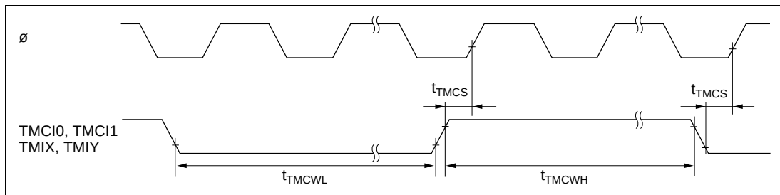
Figure 25.19 8-Bit Timer Clock Input Timing
