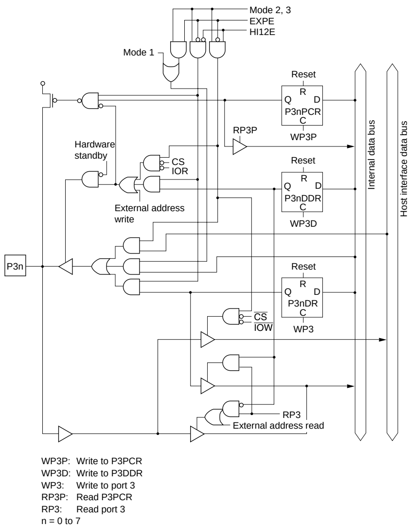
Figure C.5 Port 3 Block Diagram
