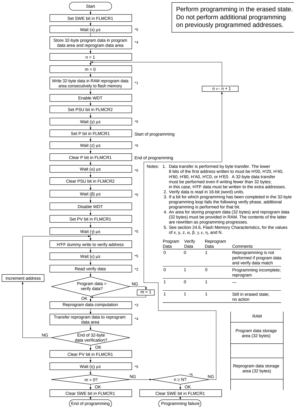
Figure 21.12 Program/Program-Verify Flowchart
