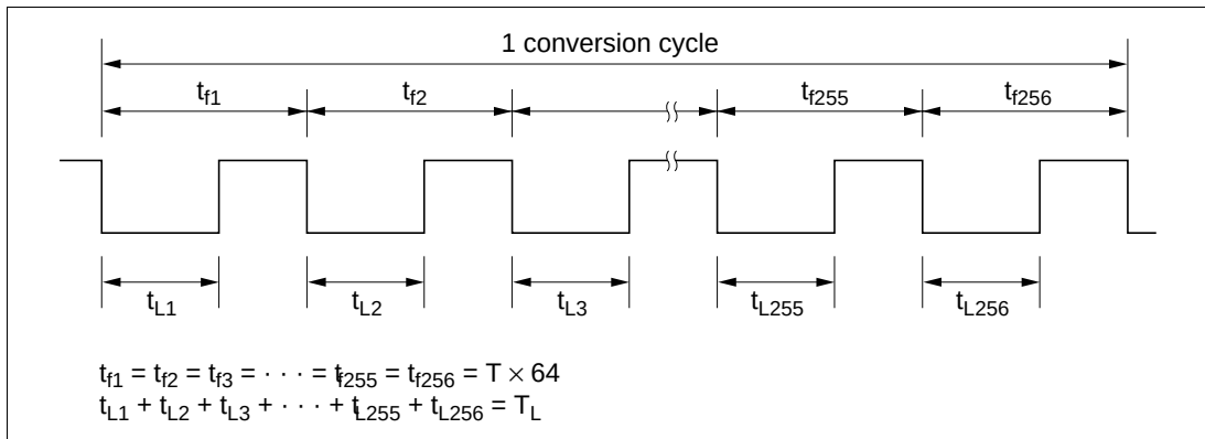
Figure 10.4 (1) Output Waveform
