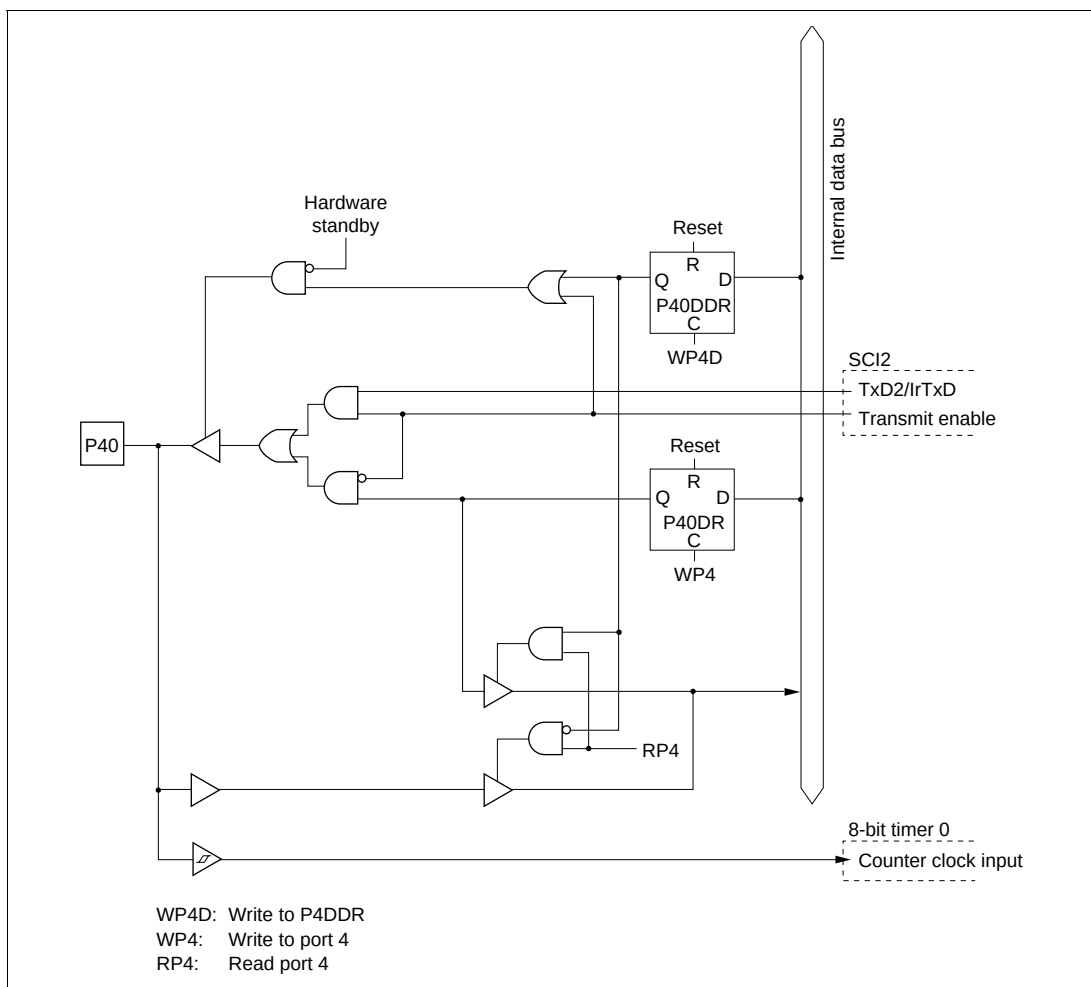
Figure C.6 Port 4 Block Diagram (Pin P40)
