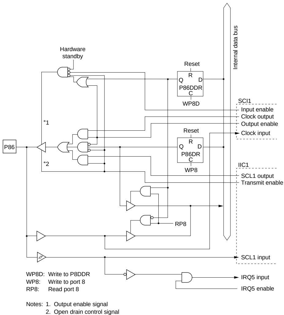
Figure C.28 Port 8 Block Diagram (Pin P86)
