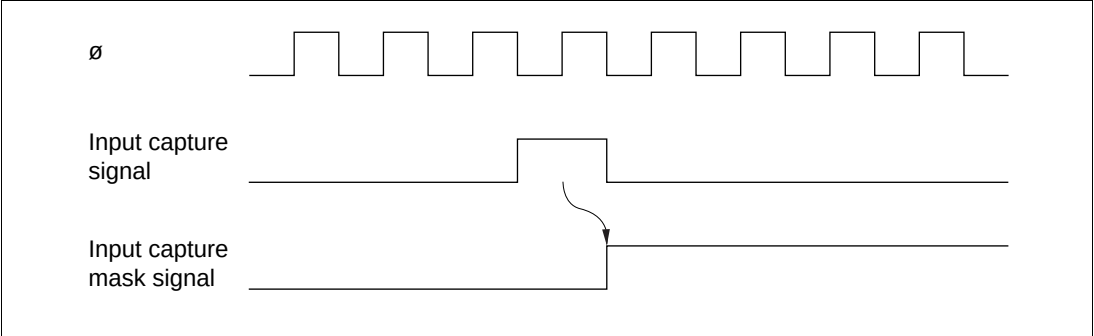
Figure 11.15 Input Capture Mask Signal Setting Timing
