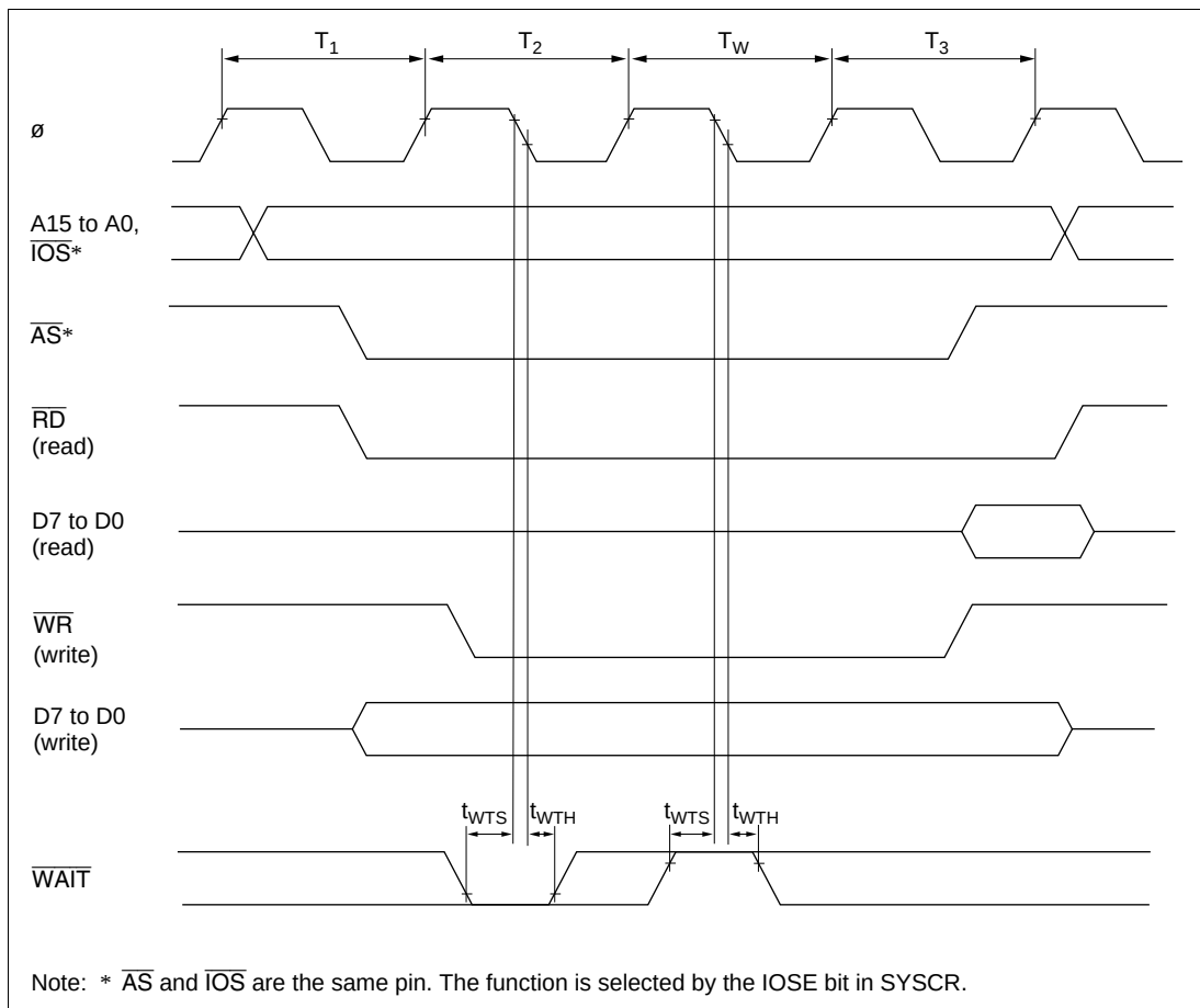
Figure 25.12 Basic Bus Timing (Three-State Access with One Wait State)
