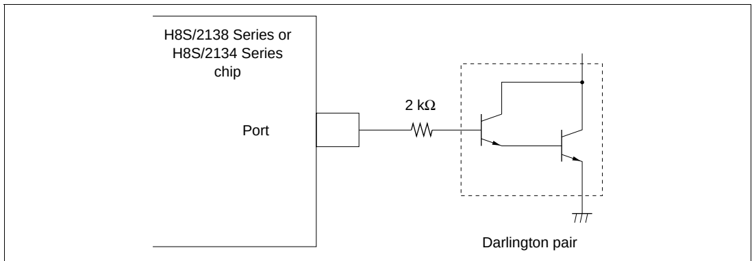
Figure 25.1 Darlington Pair Drive Circuit (Example)
