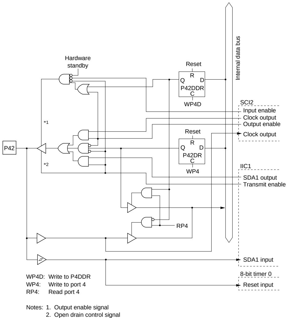
Figure C.8 Port 4 Block Diagram (Pin P42)
