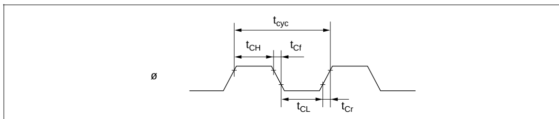
Figure 25.5 System Clock Timing
