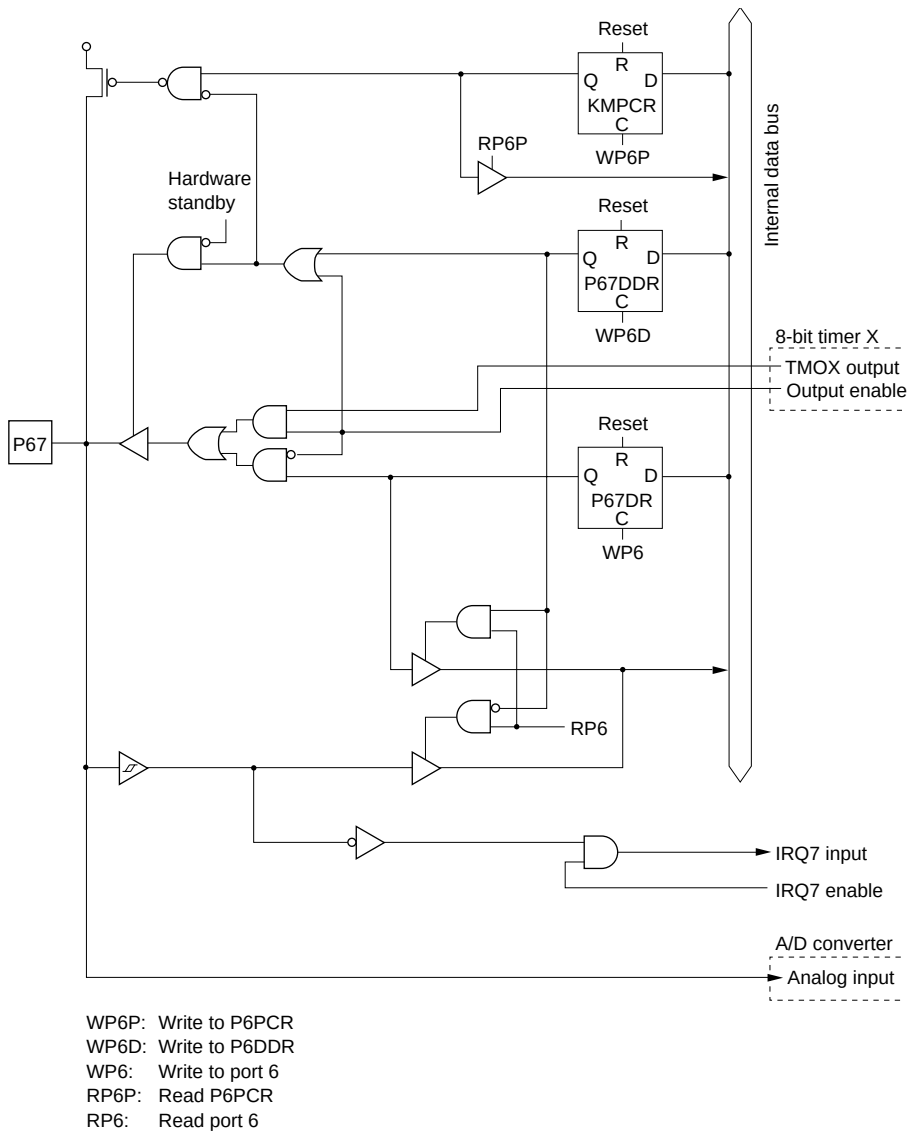
Figure C.20 Port 6 Block Diagram (Pin P67)
