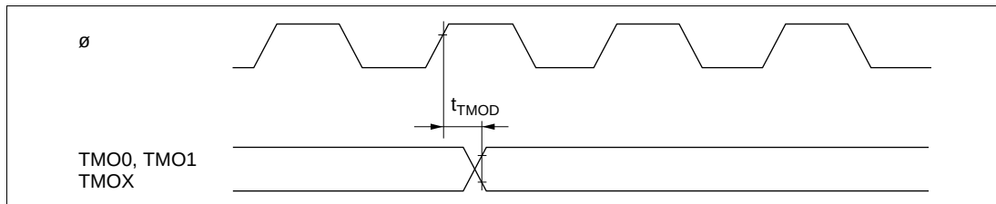
Figure 25.18 8-Bit Timer Output Timing
