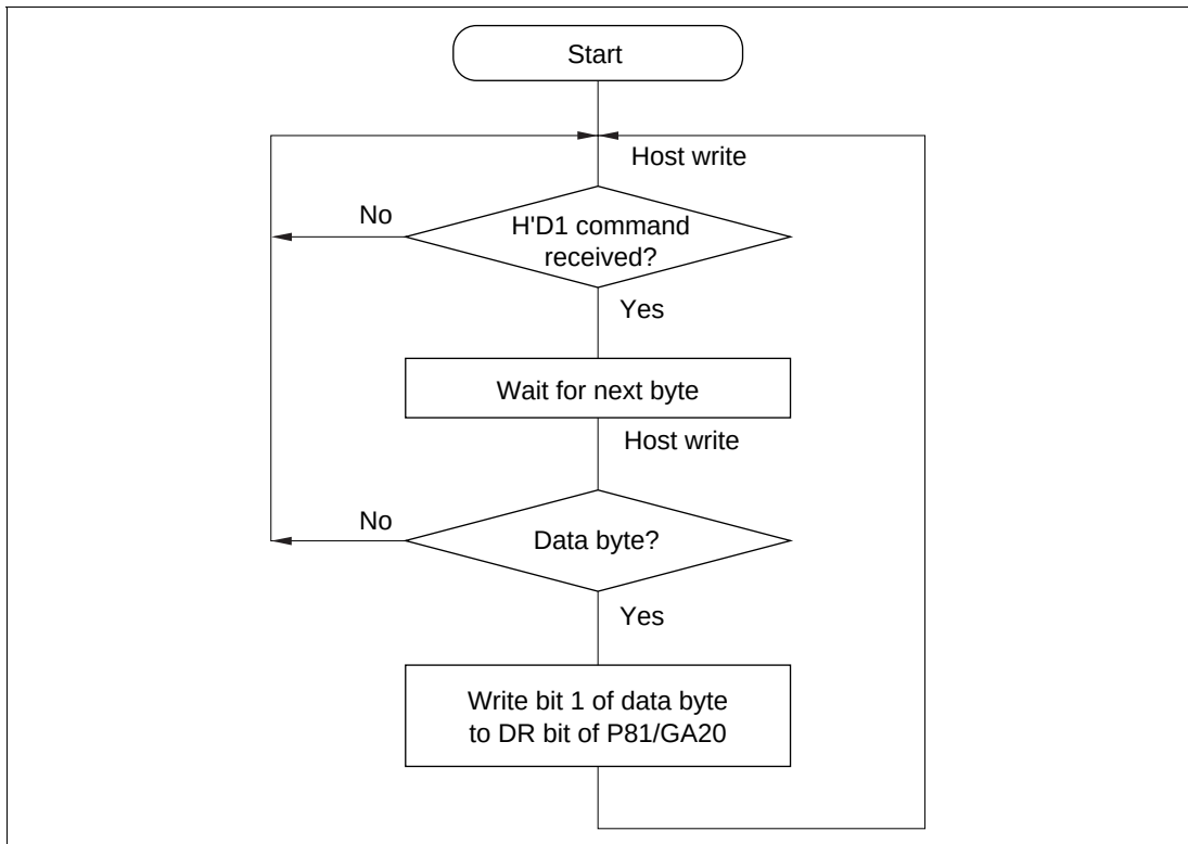
Figure 17.2 GA20 Output
