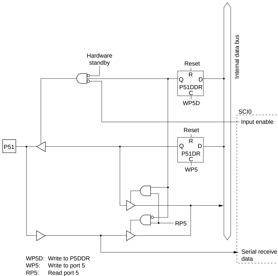
Figure C.14 Port 5 Block Diagram (Pin P51)
