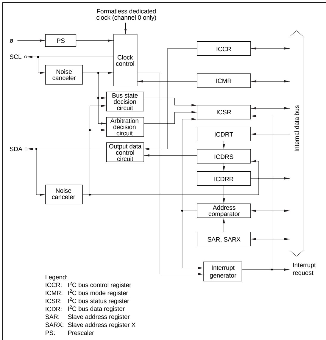
Figure 16.1 Block Diagram of I²C Bus Interface
