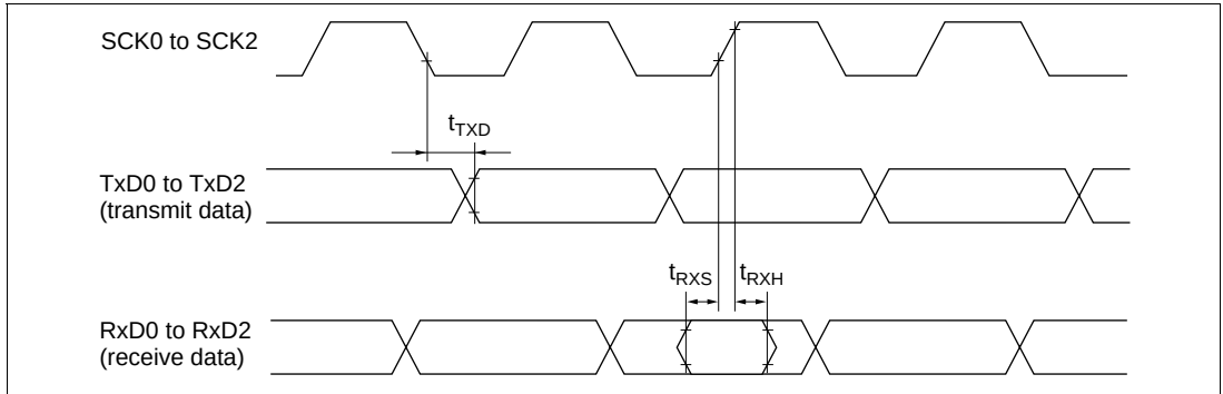
Figure 25.23 SCI Input/Output Timing (Synchronous Mode)
