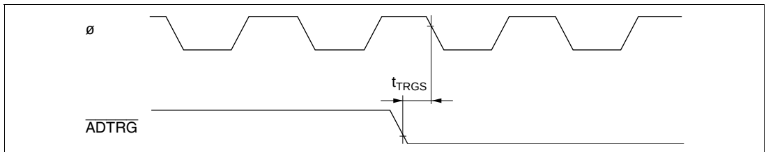
Figure 25.24 A/D Converter External Trigger Input Timing
