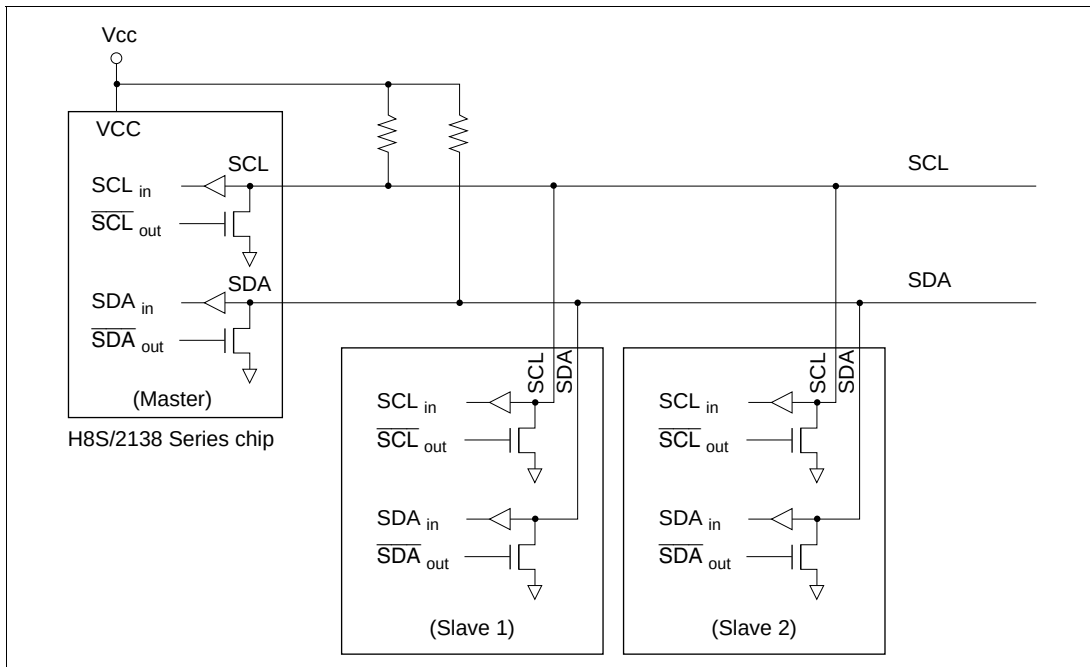
Figure 16.2 I²C Bus Interface Connections (Example: H8S/2138 Series Chip as Master)
