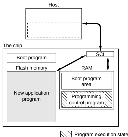
Figure 22.4 Boot Mode
