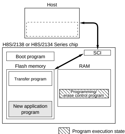
Figure 21.5 User Program Mode (Example)
