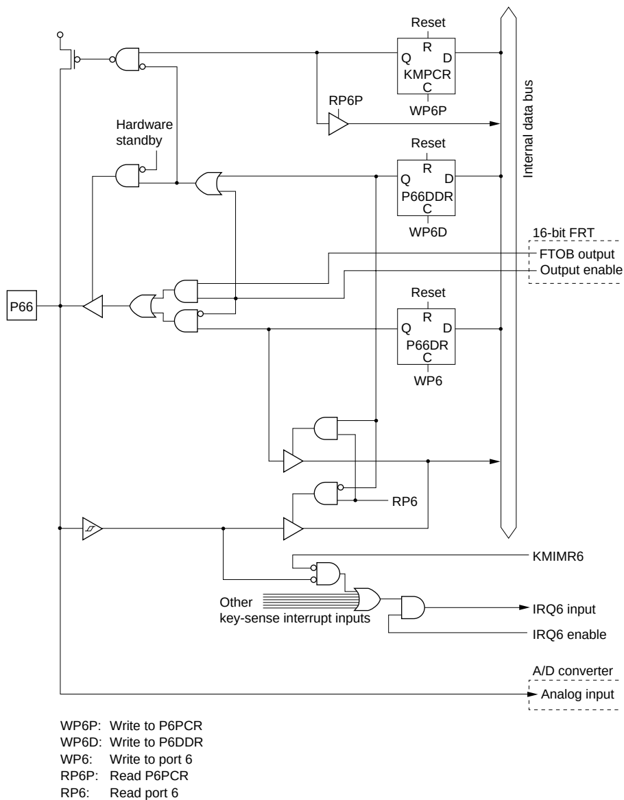
Figure C.19 Port 6 Block Diagram (Pin P66)
