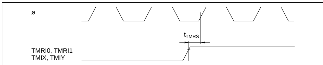
Figure 25.20 8-Bit Timer Reset Input Timing
