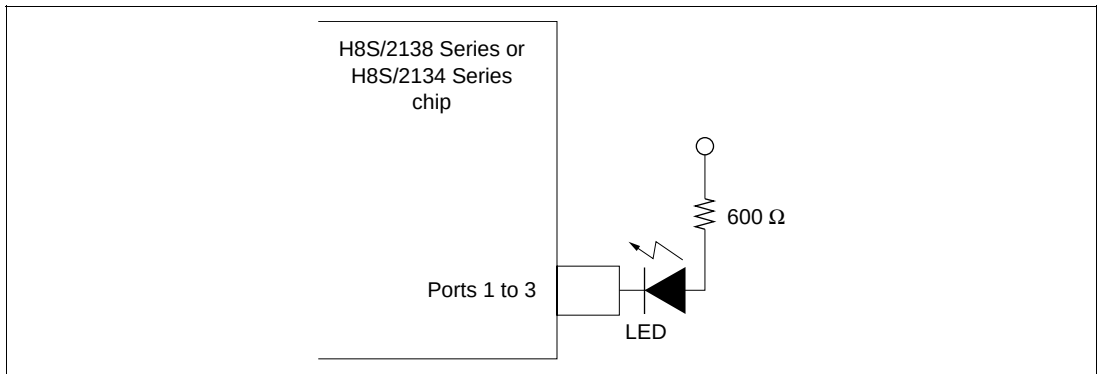
Figure 25.2 LED Drive Circuit (Example)
