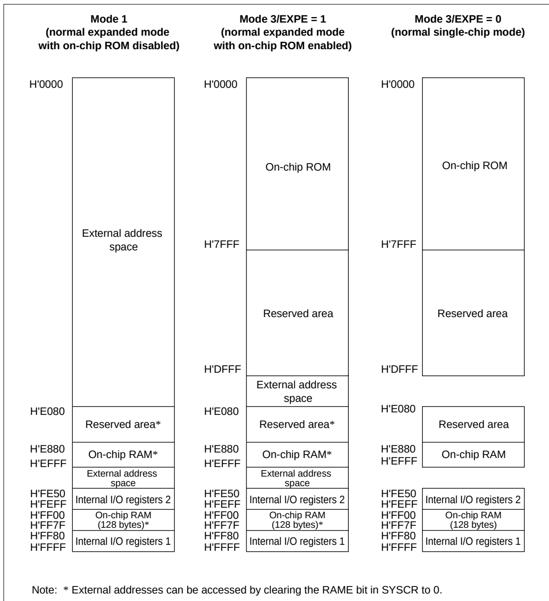
Figure 3.5 H8S/2130 Memory Map in Each Operating Mode
