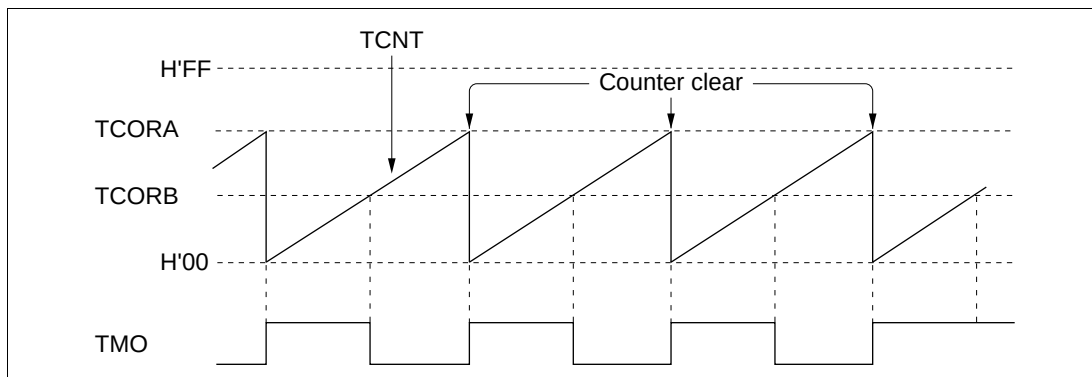
Figure 12.12 Pulse Output (Example)
