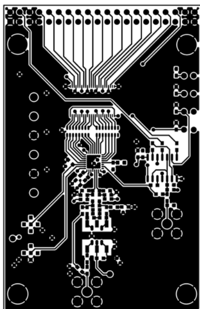
Figure 40. LFCSP Evaluation Board Layout, Primary Side
