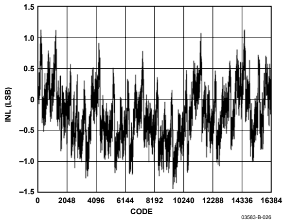
Figure 16. Typical INL
