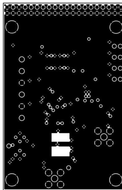
Figure 42. LFCSP Evaluation Board Layout, Ground Plane
