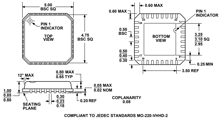
Figure 46. 32-Lead Frame Chip Scale Package [LFCSP] (CP-32-1) Dimensions shown in millimeters
