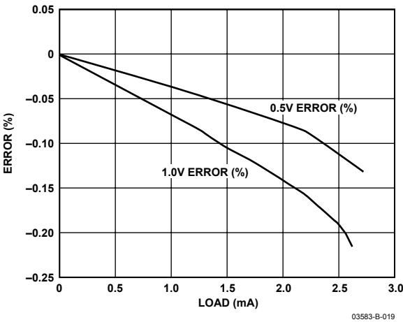
Figure 34. VREF Accuracy vs. Load
