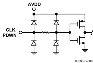
Figure 7. Equivalent Digital Input Circuit
