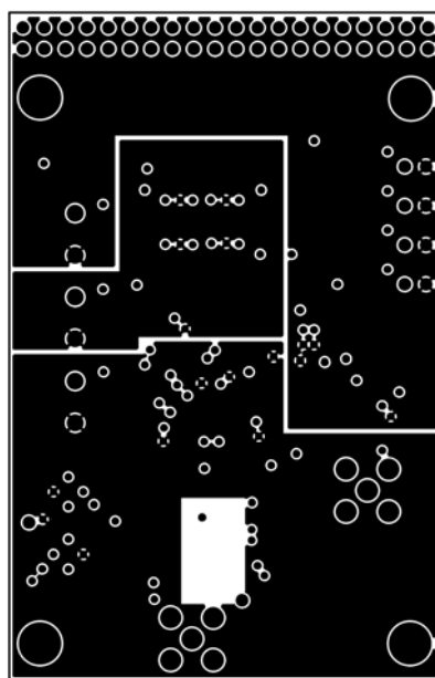
Figure 43. LFCSP Evaluation Board Layout, Power Plane
