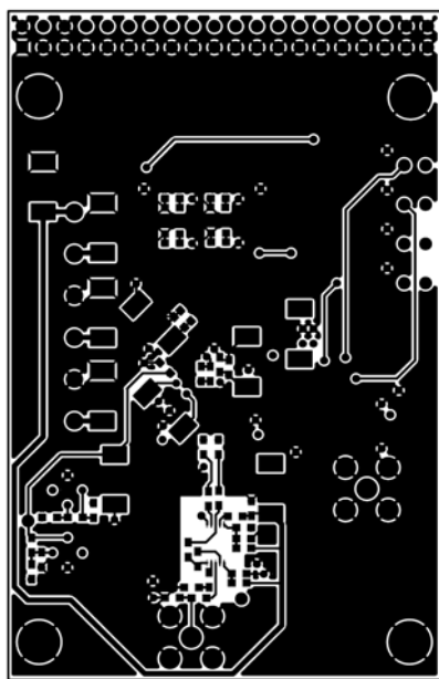
Figure 41. LFCSP Evaluation Board Layout, Secondary Side
