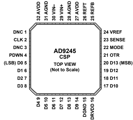
Figure 3. 32-Lead LFCSP
