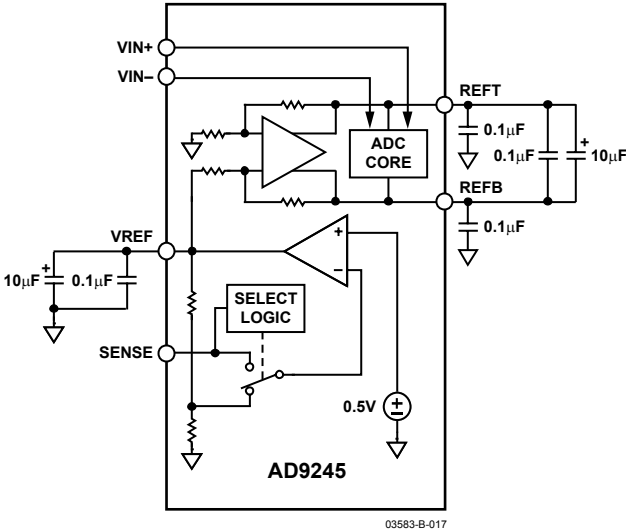
Figure 33. Internal Reference Configuration
