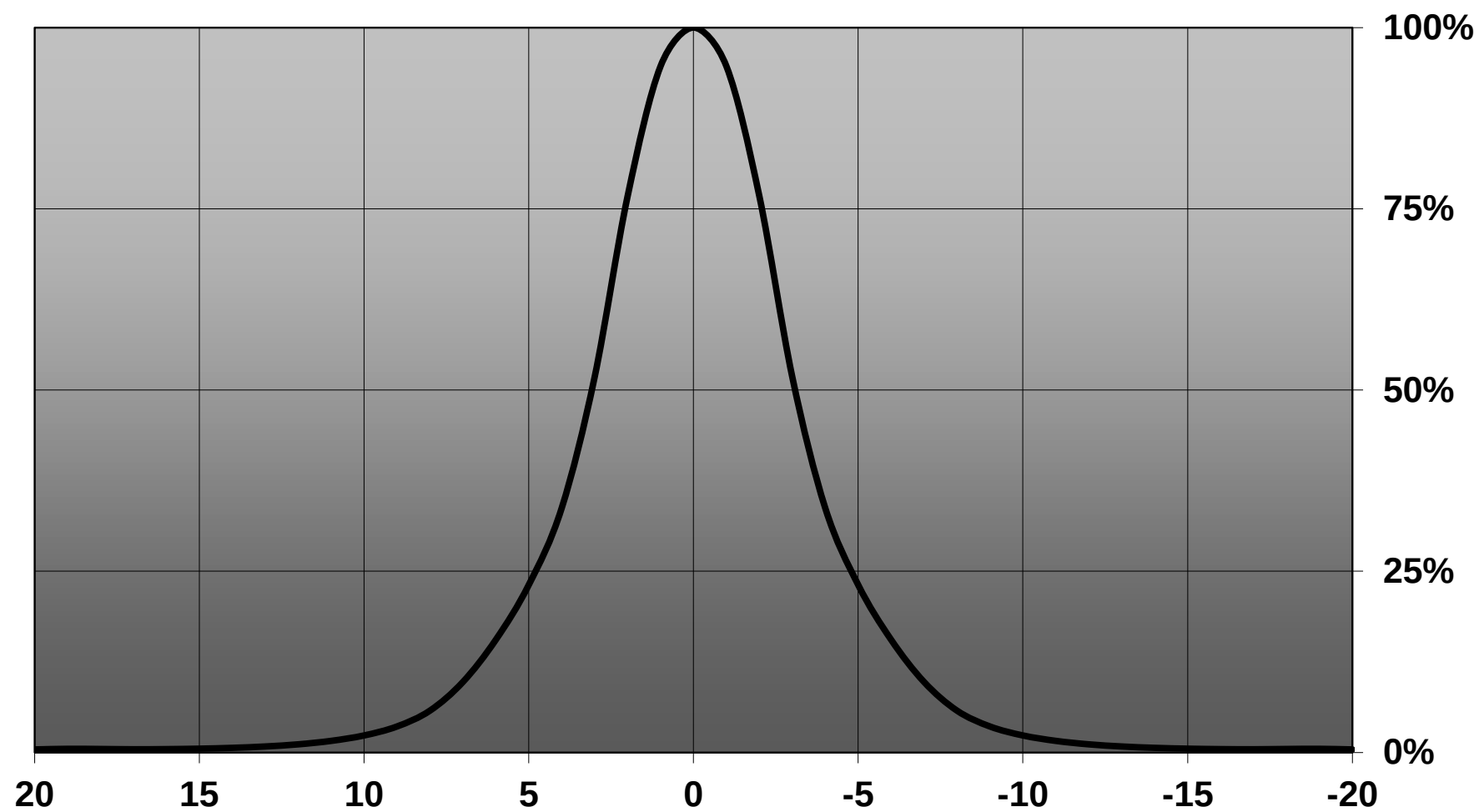
Relative intensity of C4F12077_Iris-XP-G-tape
