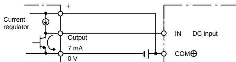
NPN open-collector output
