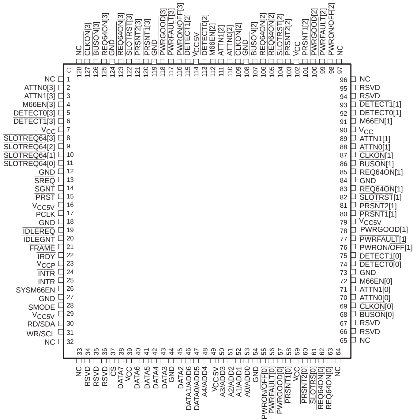
PBK LOW-PROFILE QUAD FLAT PACKAGE
