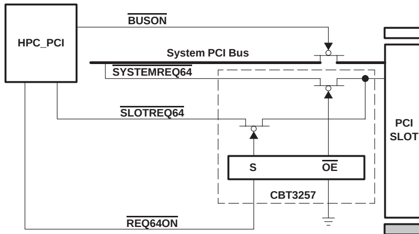
Figure 13. \text{SLOTREQ64} Implementation Using CBT3257
