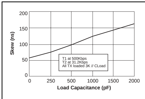
Figure 1. Transmitter Skew VS. Load Capacitance for the 3223EU / 3243EU
