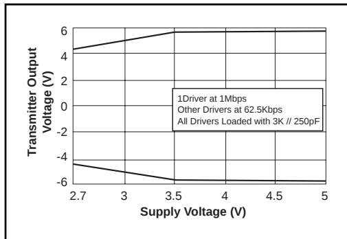
Figure 2. Transmitter Output Voltage VS. Supply Voltage for the SP3223EU
