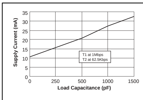
Figure 4. Supply Current VS. Load Capacitance for the SP3223EU
