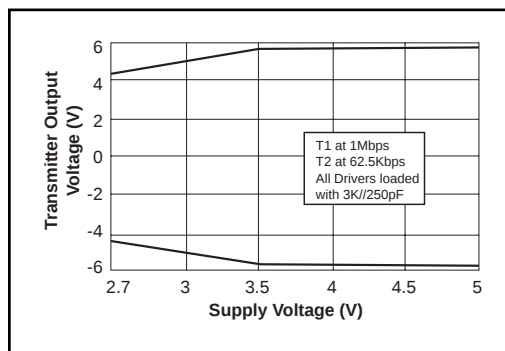
Figure 6. Transmitter Output Voltage VS. Supply Voltage for the SP3223EU
