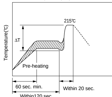
Dip Soldering/Soldering Iron Conditions (Example)
