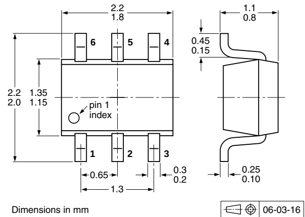
Fig 8. Package outline BAV99S (SOT363/SC-88)
