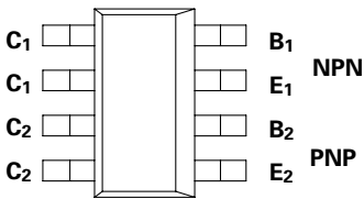
PARTMARKING DETAIL – T6718
