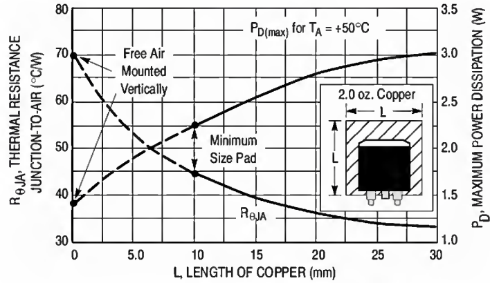
FIGURE 6 – D²PAK Thermal Resistance and Maximum Power Dissipation vs. P.C.B Copper Length
