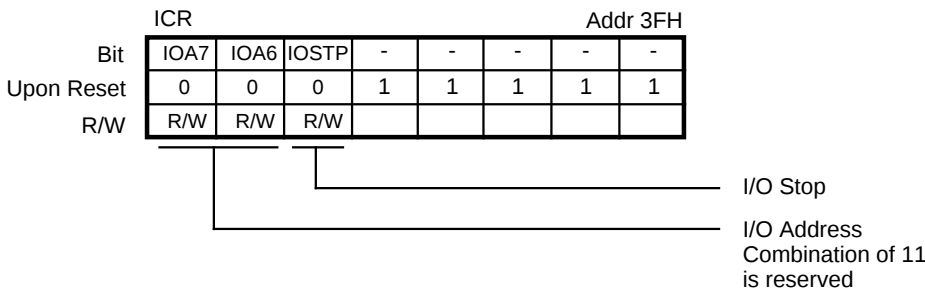
Figure 50. I/O Control Register
