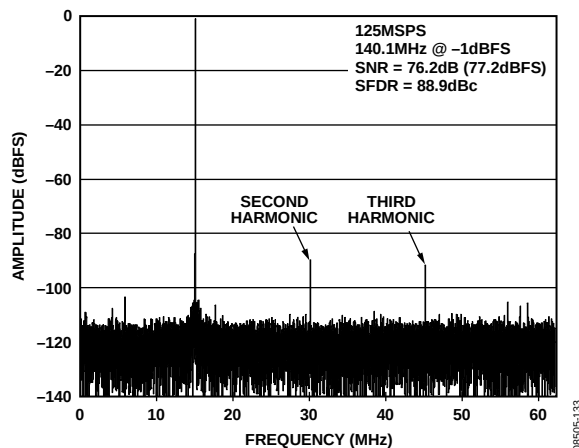
Figure 33. AD9255-125 Single-Tone FFT with f_{IN} = 140.1 MHz
