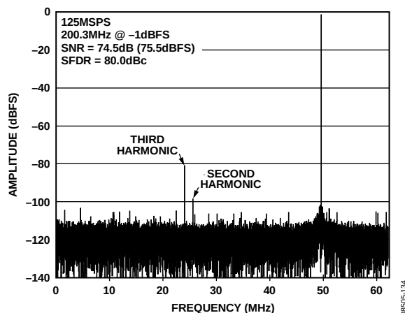
Figure 34. AD9255-125 Single-Tone FFT with f_{IN} = 200.3 MHz
