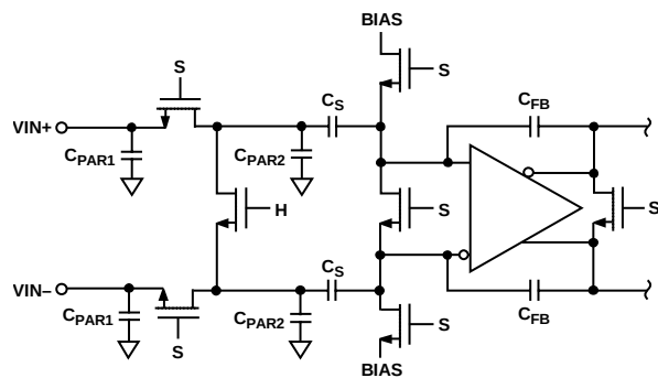
Figure 64. Switched-Capacitor Input
