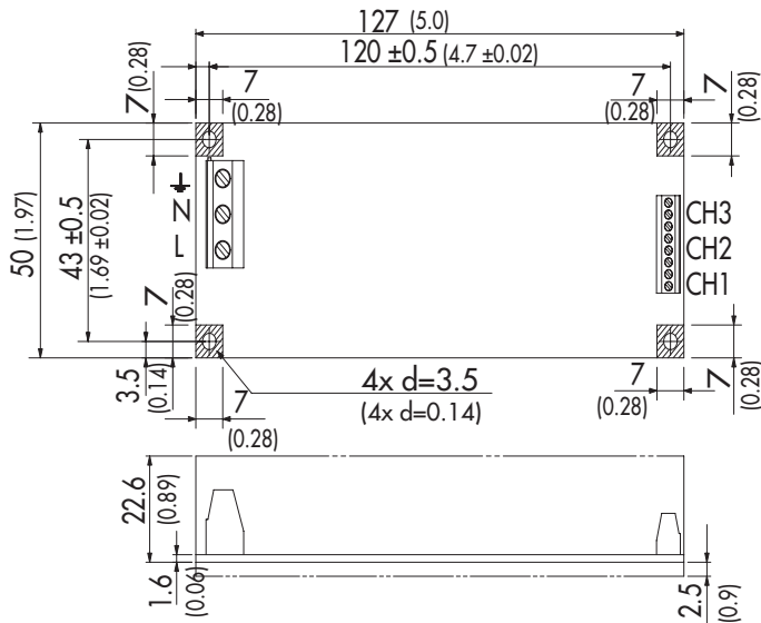
TOF 15-T standard open frame version
