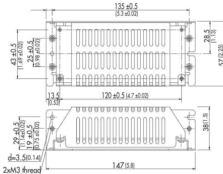
TOF 15-T with chassis / cover option
