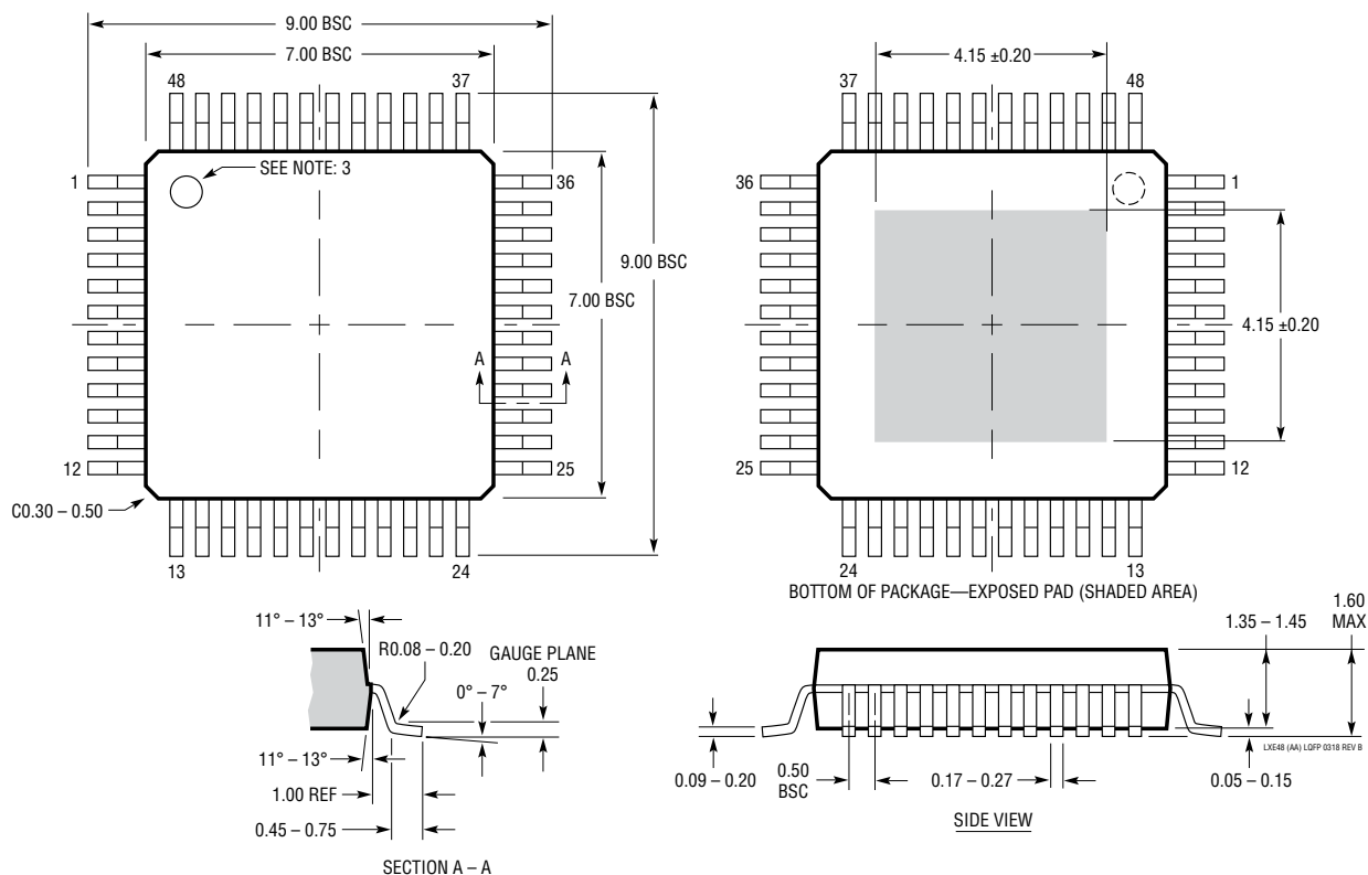
LXE Package 48-Lead Plastic Exposed Pad LQFP (7mm × 7mm) (Reference LTC DWG #05-08-1927 Rev B) Exposed Pad Variation AA
