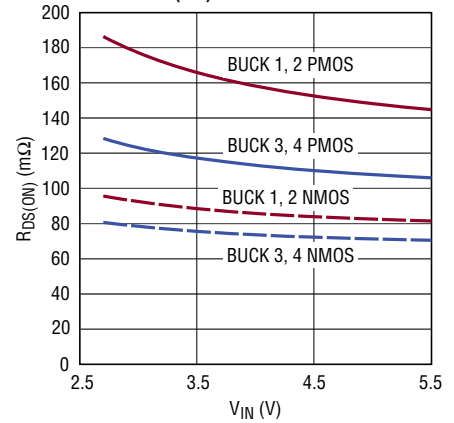
Buck R_{DS(ON)} vs V_{IN}
