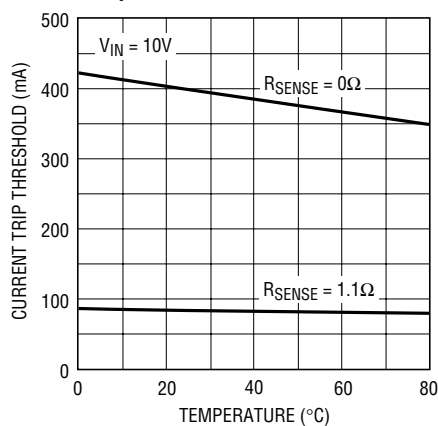
Current Trip Threshold vs Temperature
