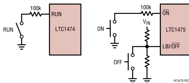
Figure 7. Simplified Implementation of LTC1474 and LTC1475 On/Off
