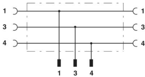
Circuit diagram
