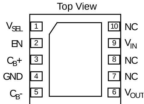
Figure 3. Pin Assignments
