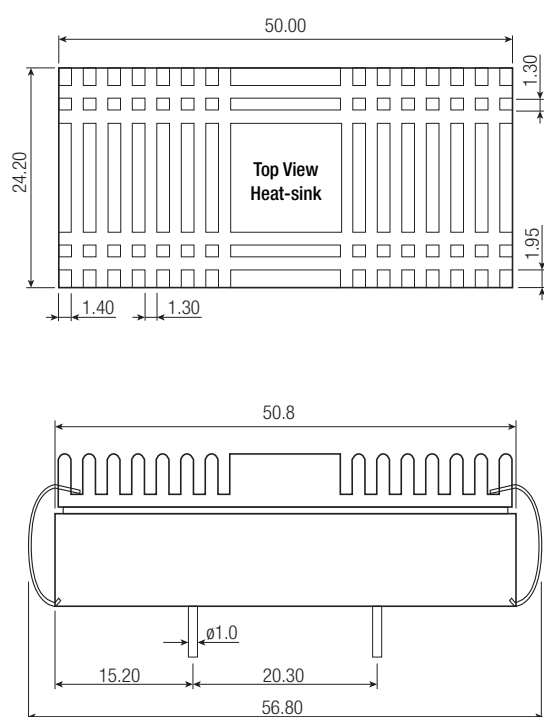
Dimension Drawing (mm) with Heat-sink
