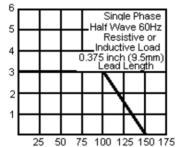
Maximum Forward Current Derating Curve
